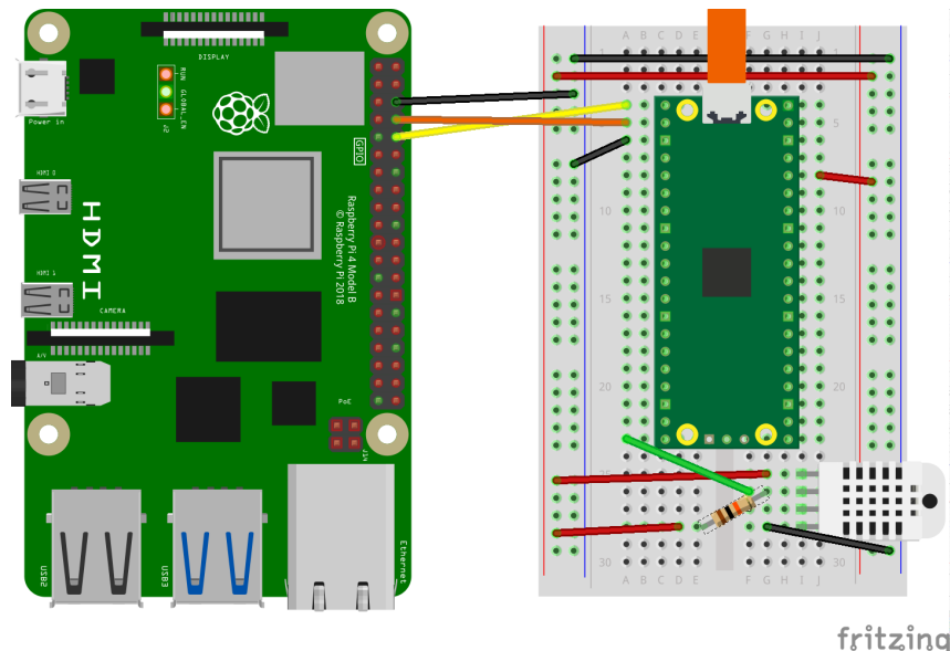
Figure 10. Wiring the DHT-22 temperature sensor to Raspberry Pi Pico, and connecting Pico's UART0 to the Raspberry Pi 4.
