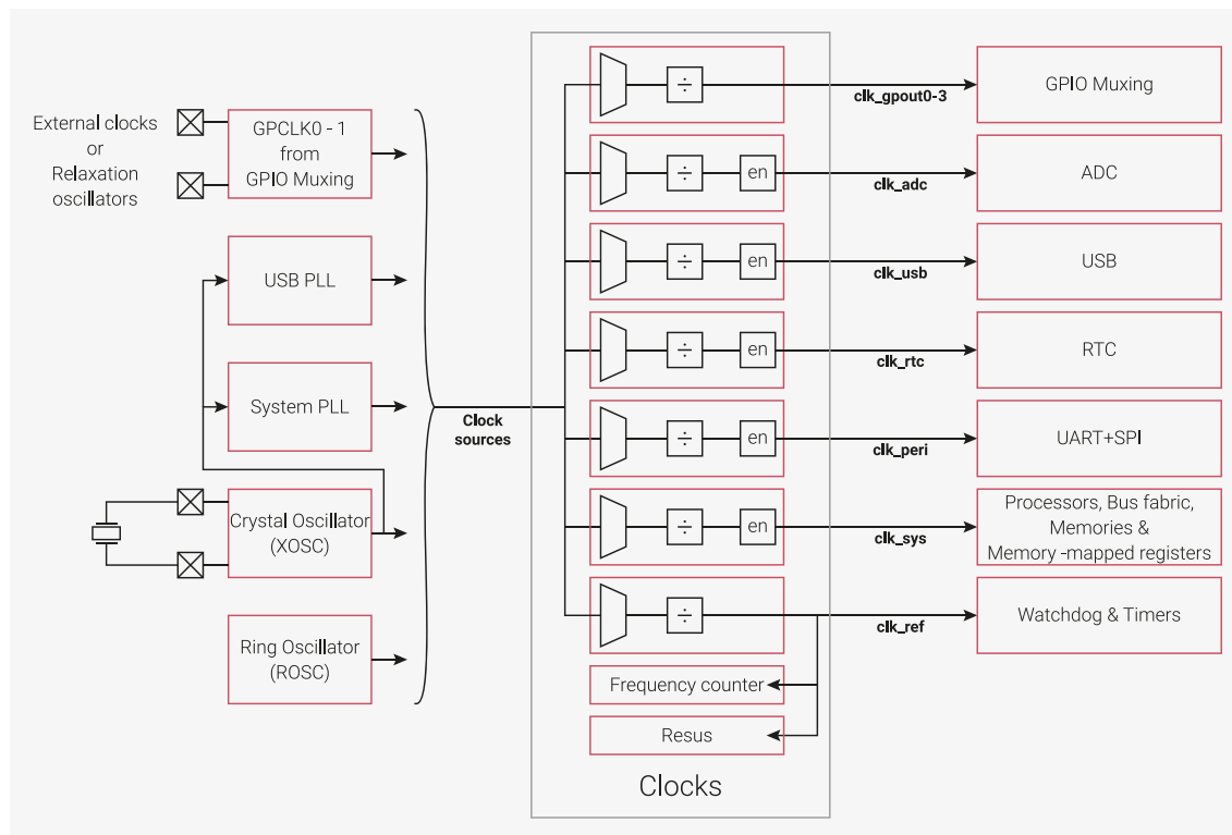
Figure 28. Clocks overview
